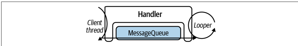
Figure 4-5. Looper/Handler .
