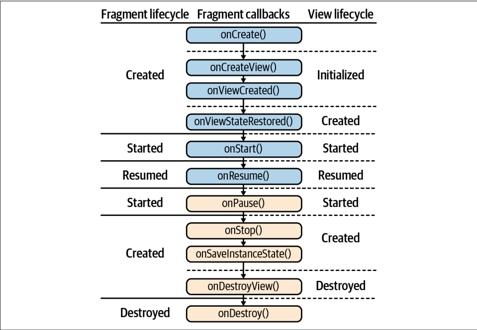
Figure 3-3. Fragment lifecycle.
