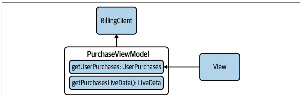
Figure 6-1. MVVM architecture.
