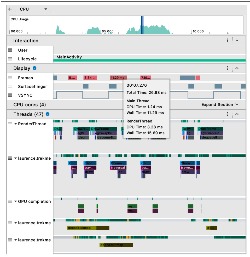
Figure 11-19. System Trace reveals dropped frames where times are labeled within Frames.
