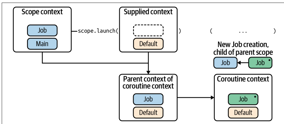
Figure 7-11. Context detail.
