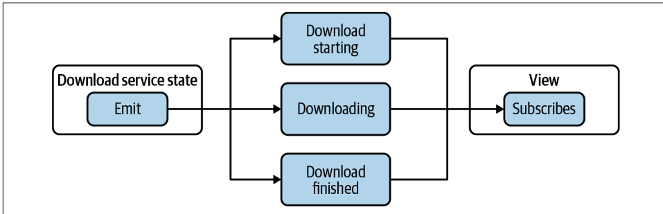
Figure 10-11. Download state.
